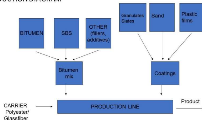
PRODUCTION DIAGRAM
